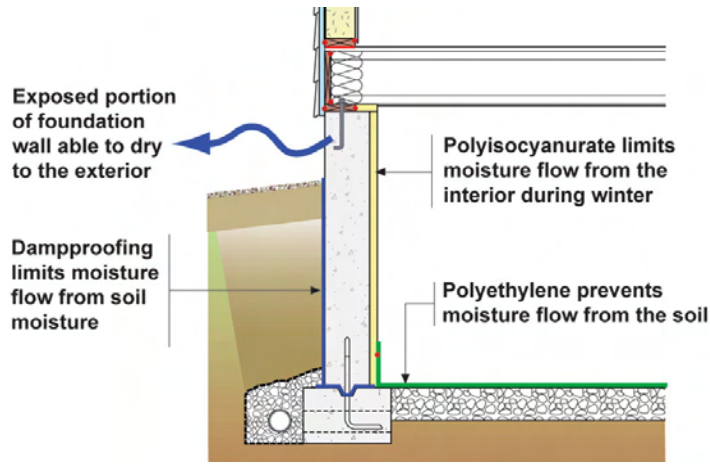
Figure 19: Foundation Vapor Management
