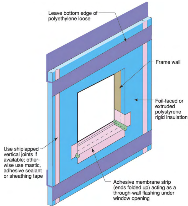
Figure 13: Drainage plane and Window Flashing
