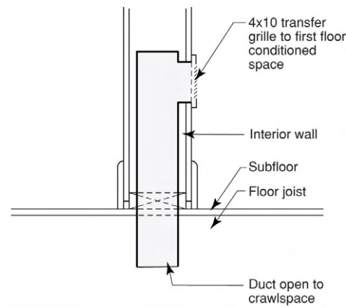
Figure 27: Transfer Grille to Crawlspace
