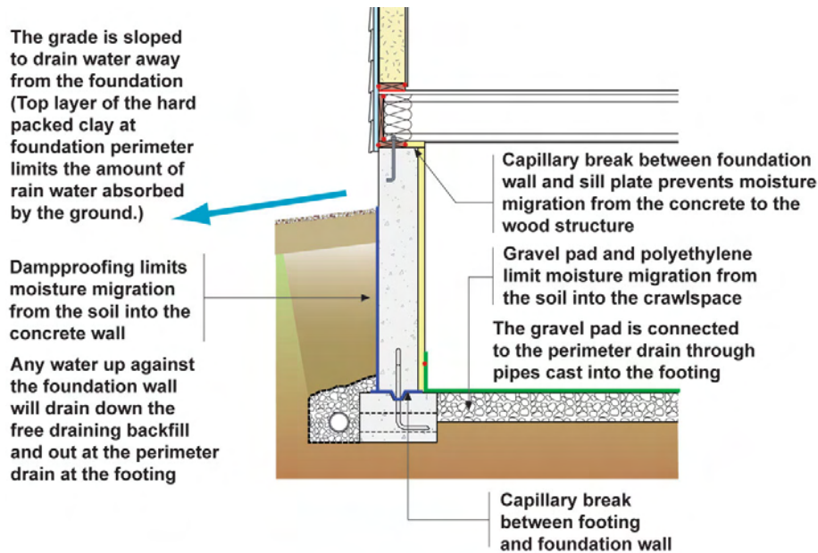
Figure 17: Foundation Drainage
