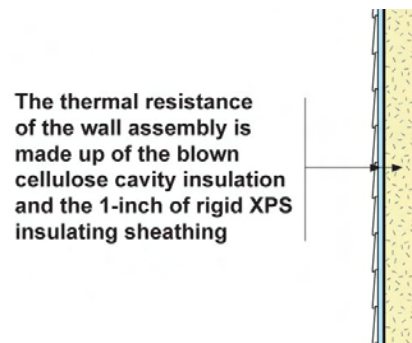
Figure 16: Wall Thermal Resistance
