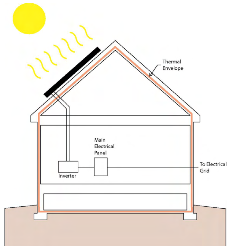
Figure 32: Schematic of a Photovoltaic System
