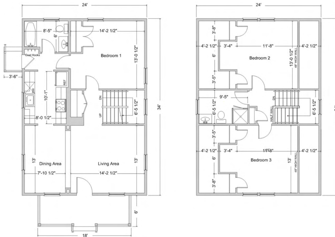
Figure 2: Mixed-Humid floor plans (Right: Ground Floor, Left: Second Floor, crawlspace not shown)
