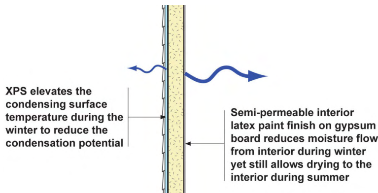
Figure 15: Wall Vapor Management
