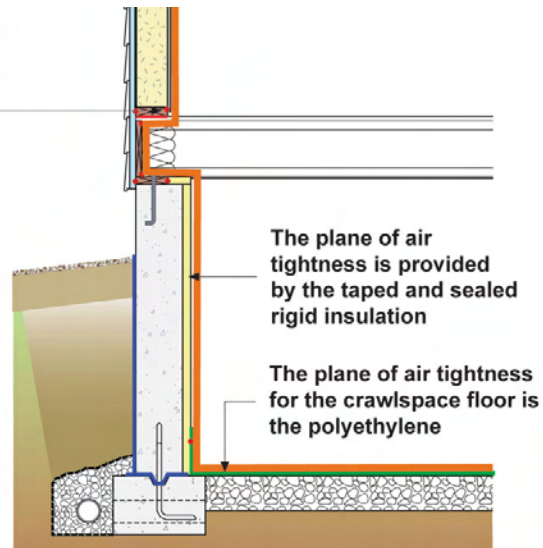
Figure 18: Foundation Air Barrier
