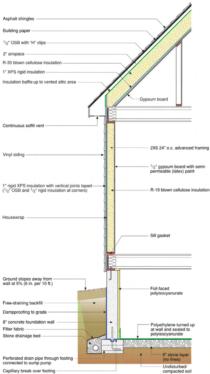
Figure 5: Building Section
