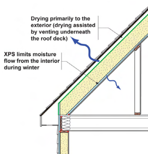
Figure 10: Roof Vapor Management
