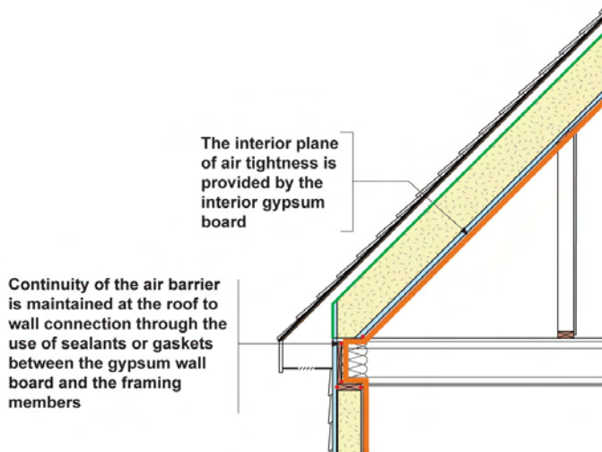
Figure 9: Roof Air Barrier
