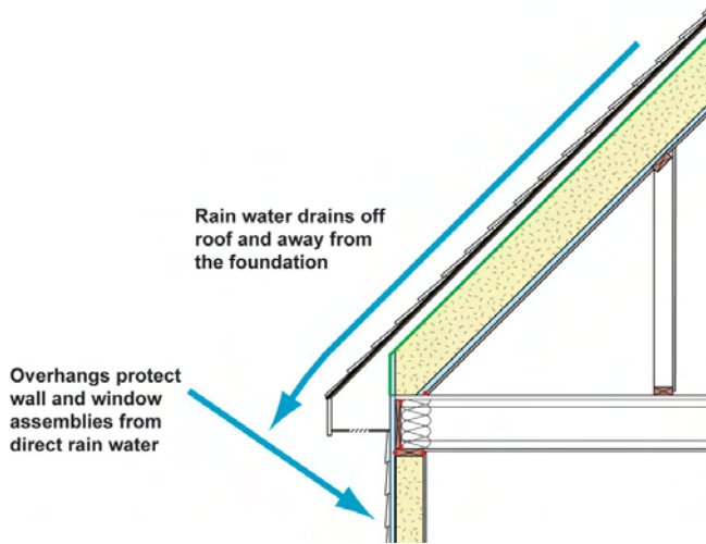
Figure 8: Roof Drainage
