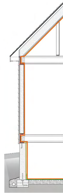
Air Barrier
