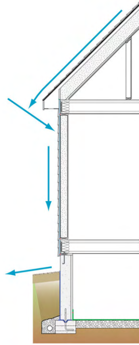
Drainage
