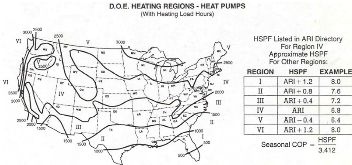
Figure 24: HSPF Adjustment Map
