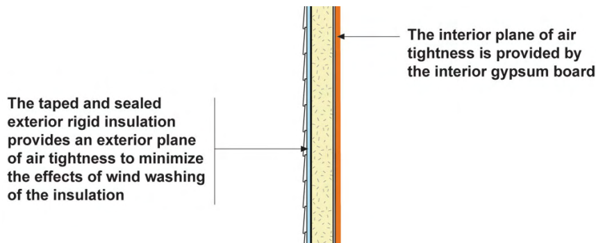
Figure 14: Wall Air Barrier
