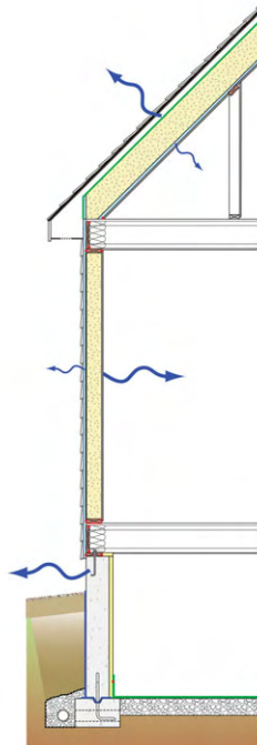
Vapor Management
