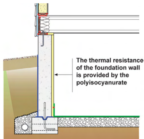
Figure 20: Foundation Thermal Resistance
