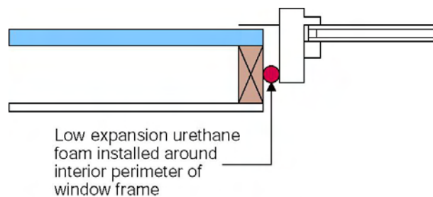
Figure 22: Window Air Barrier Continuity
