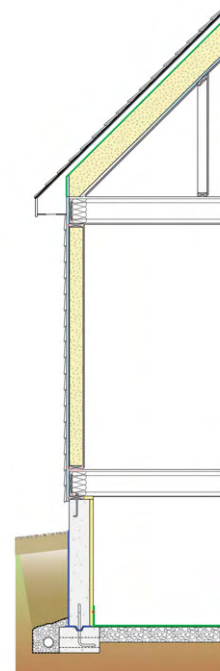
Thermal Resistance
