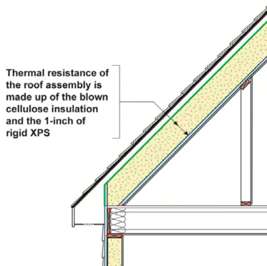
Figure 11: Roof Thermal Resistance
