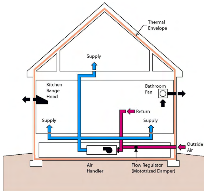
Figure 23: Mechanical Schematic for Mixed-Humid Climate House
