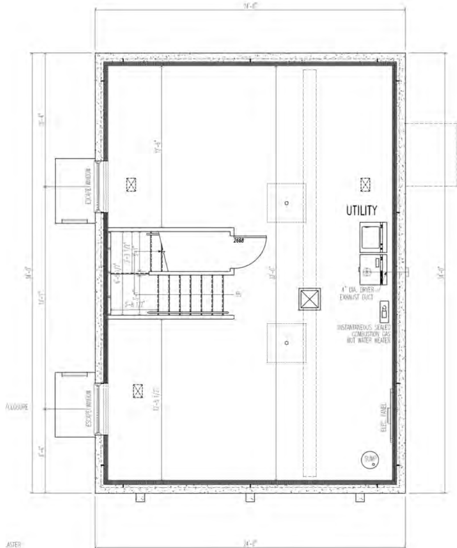
Figure 6 : Basement Floorplan of BA Westford Prototype House
