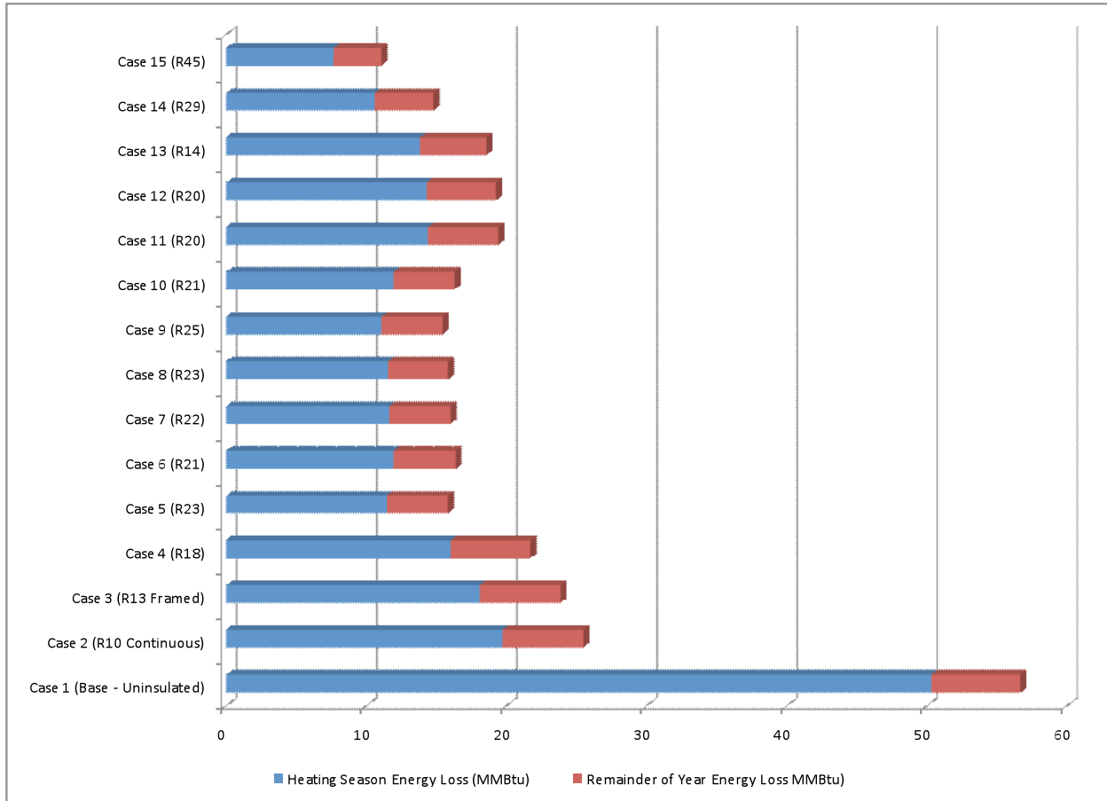
Figure 7 : Comparison of Heating Energy Losses for all Cases
