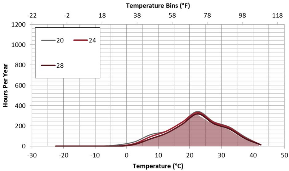
Figure 21. Biodegradation risk plot for exterior side of the sheathing, with 1 in. of exterior insulation and 50 Perm WRB and Kraft interior vapor control.
