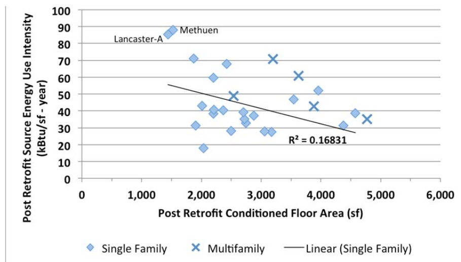
Figure 17. Source energy use intensity relative to post-retrofit conditioned floor area for comprehensive DERs
