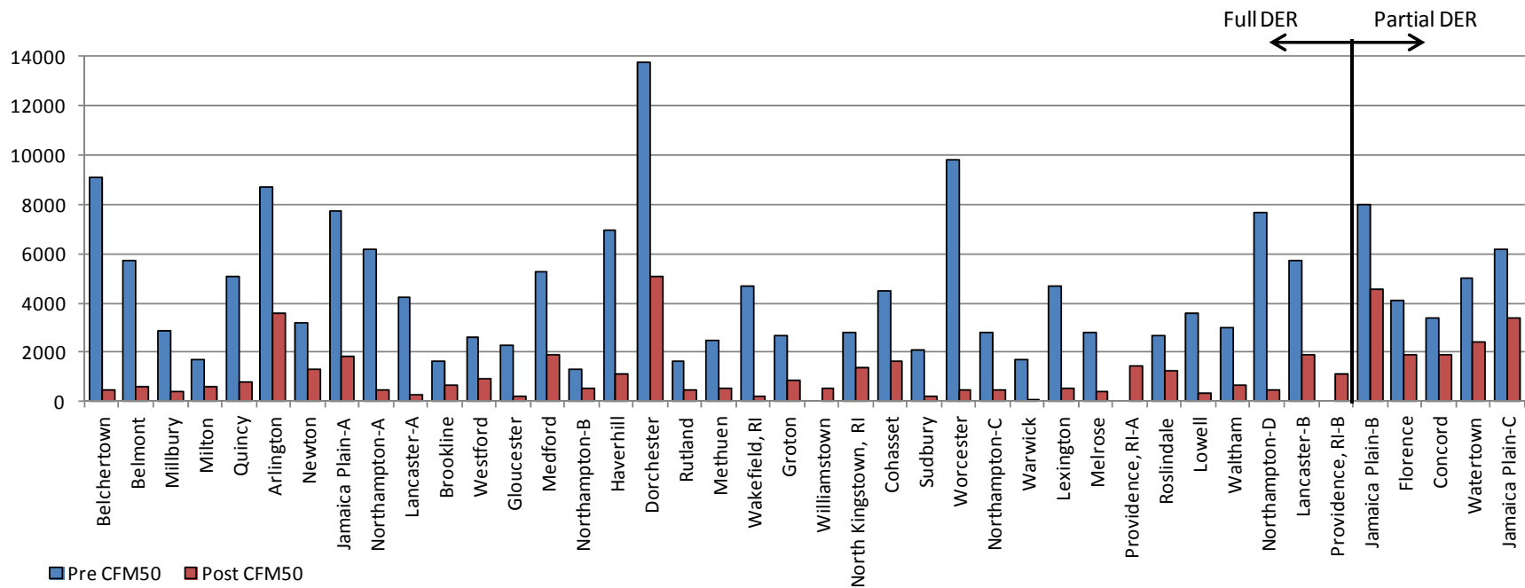
Figure 24. Pre-DER and Post-DER total CFM 50 results
