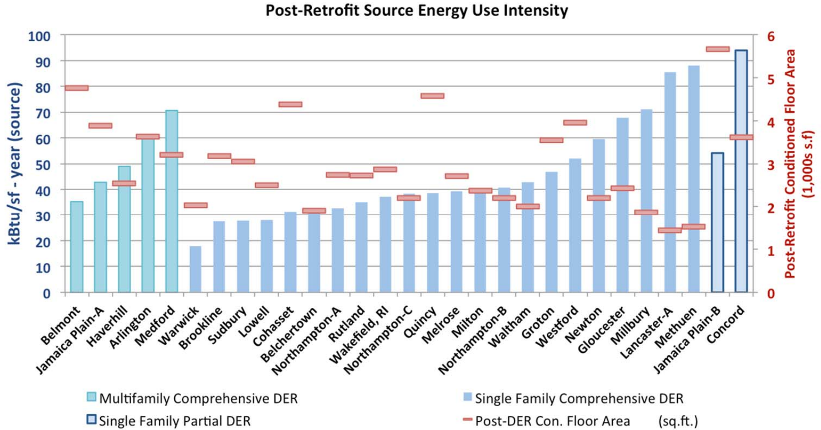
Figure 18. Post-retrofit source energy use intensity and post-retrofit conditioned floor area
