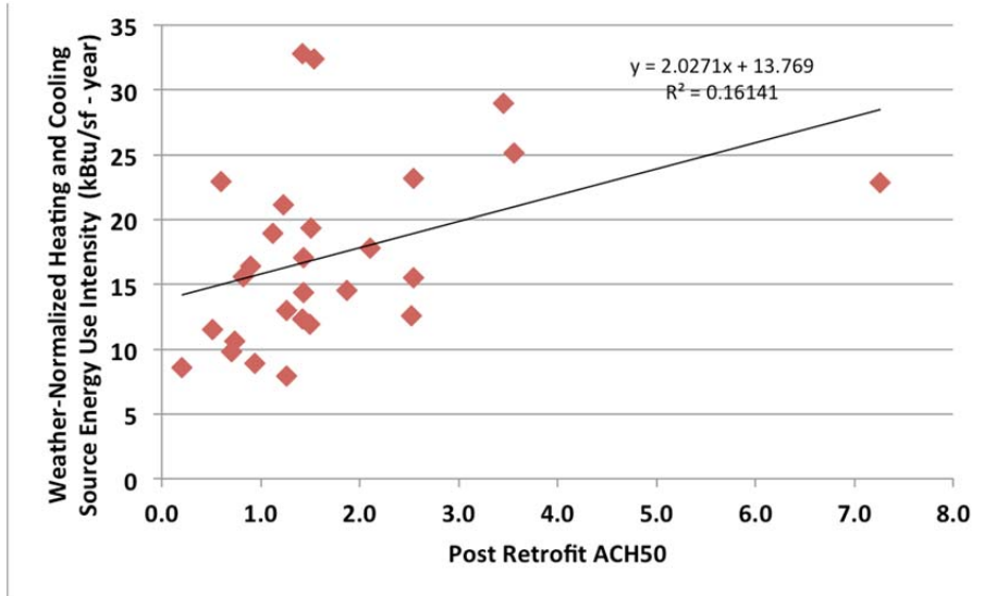
Figure 22: Post-retrofit heating and cooling energy use intensity relative to post-retrofit ACH50
