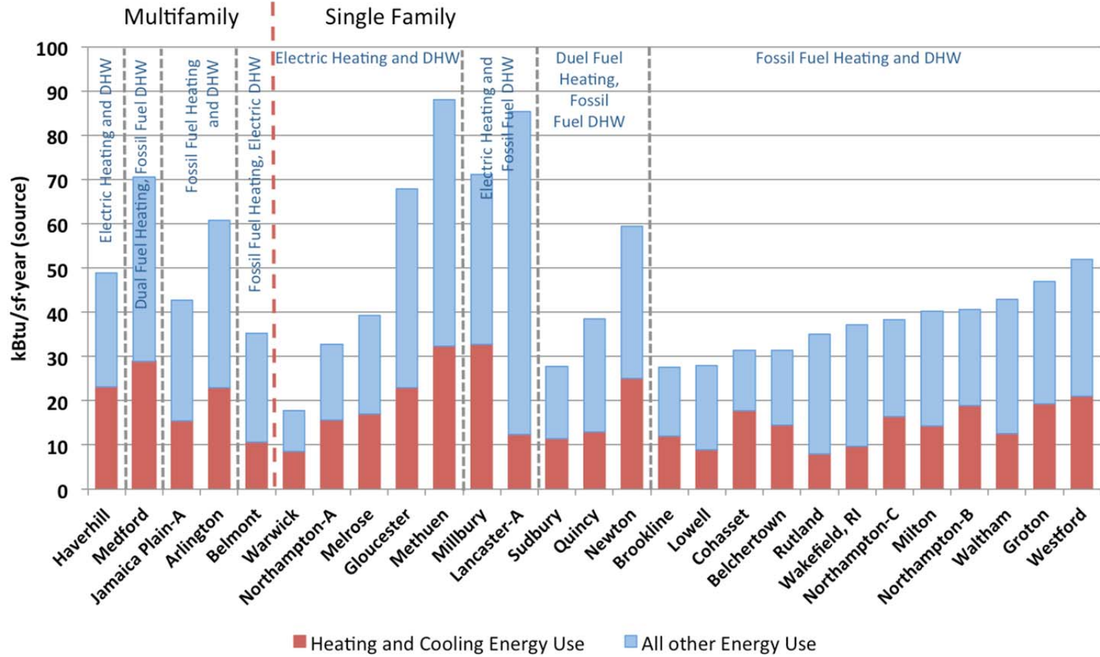
Figure 19. Post-retrofit source energy use intensity grouped by heat and DHW fuel source with post-retrofit conditioned floor area
