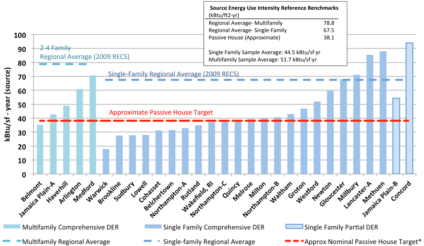
Figure 16: Post-retrofit source Energy Use Intensity (kBtu/ft²·yr)
