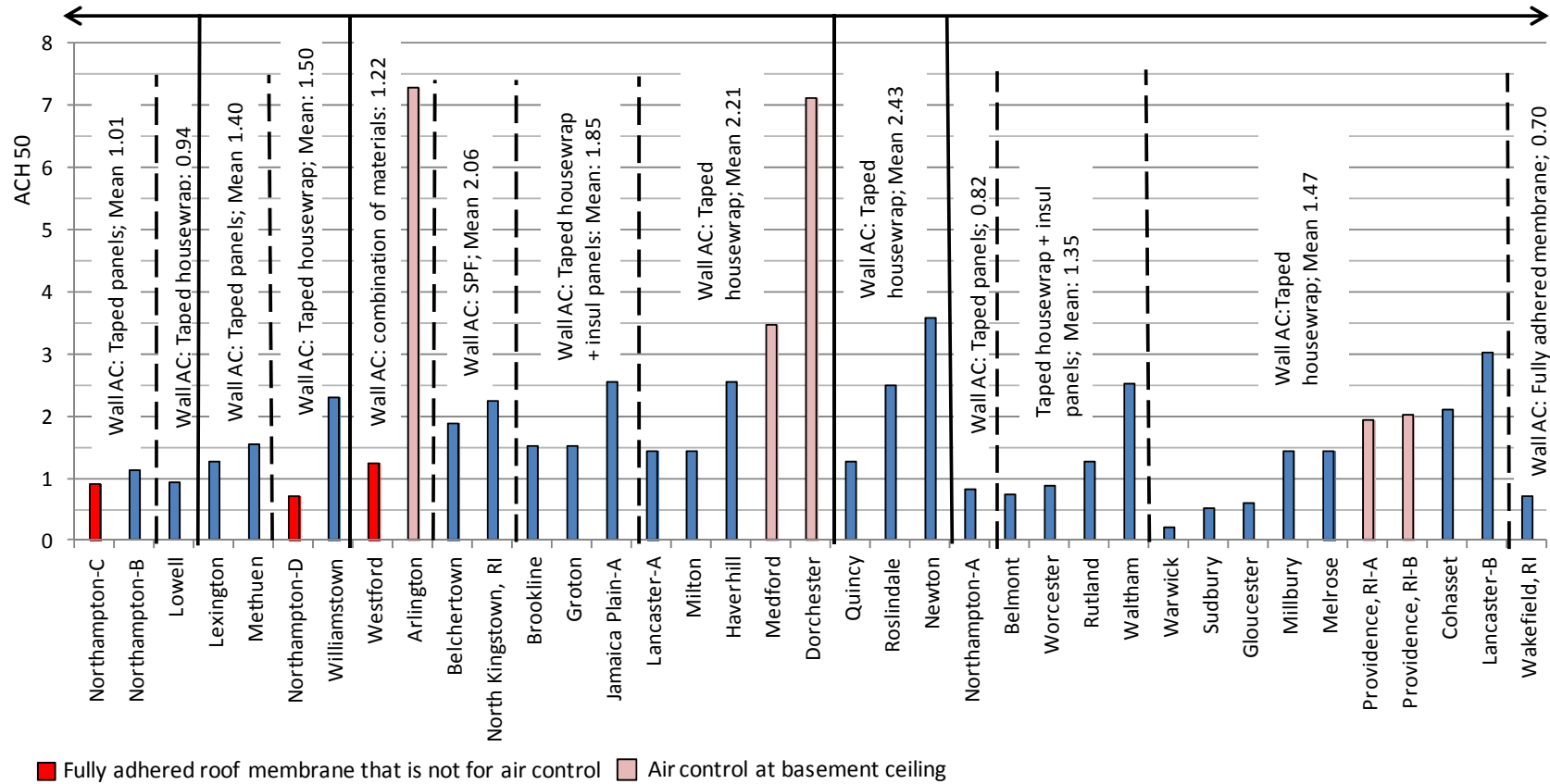
Figure 30. Post-DER ACH 50 results grouped roof and wall air control (AC) material
