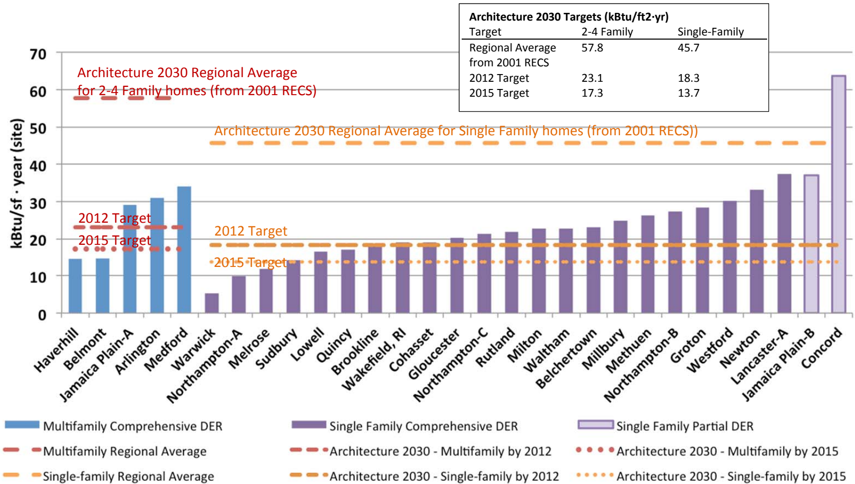
Figure 15: Post-retrofit site Energy Use Intensity (kBTu/ft 2 -yr)
