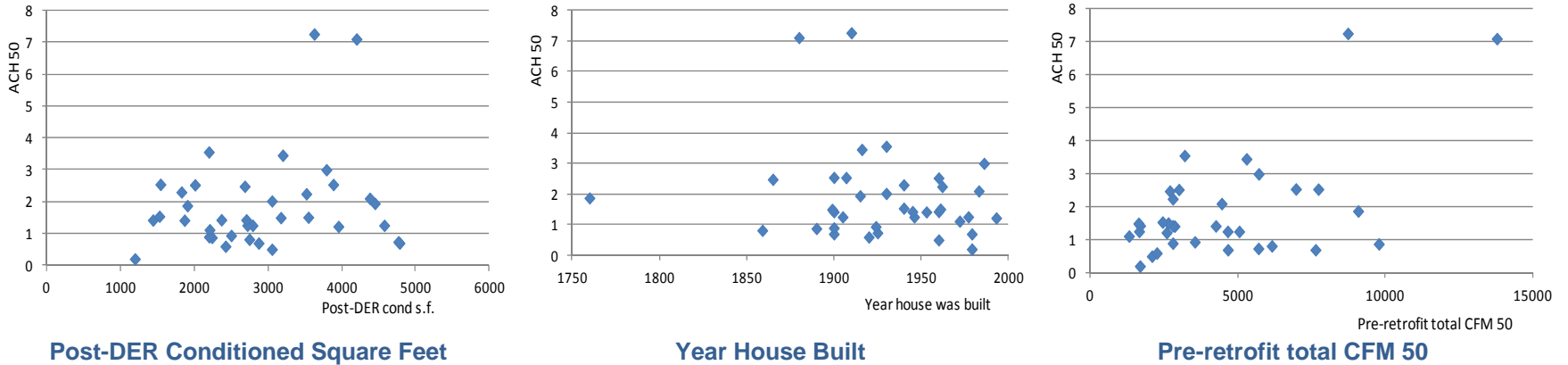
Figure 27. Post-DER ACH 50 versus size of house, year house was built, and pre-DER total CFM 50
