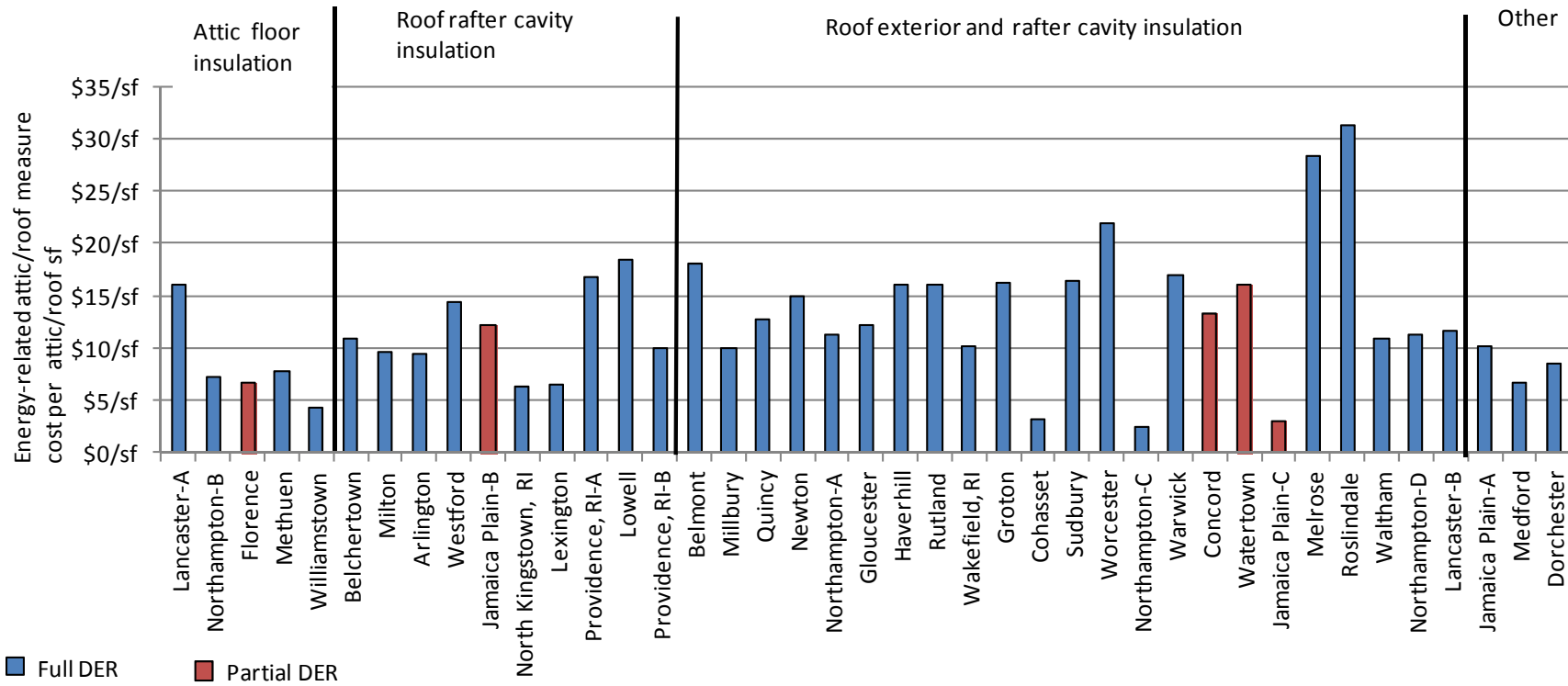
Figure 37. Total energy-related attic roof costs per attic/roof sf
