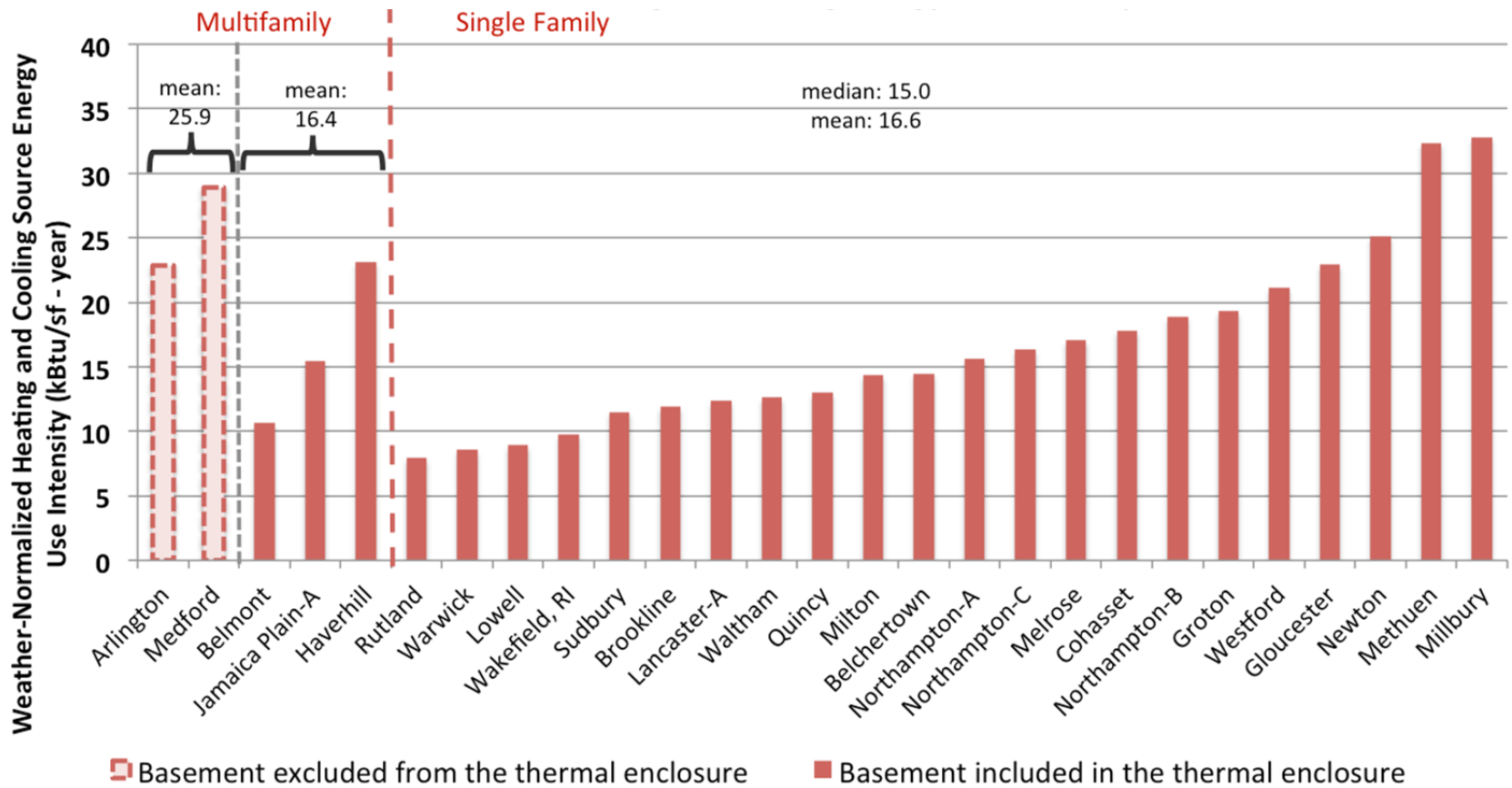
Figure 20. Post-retrofit heating and cooling source energy use intensity by basement treatment
