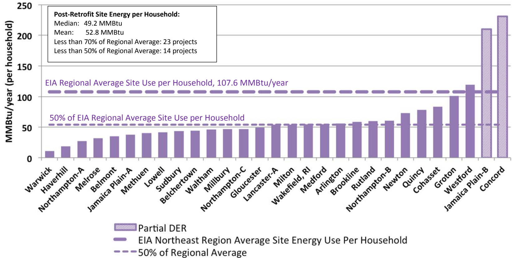
Figure 13. Post-retrofit site MMBtu/year per household
