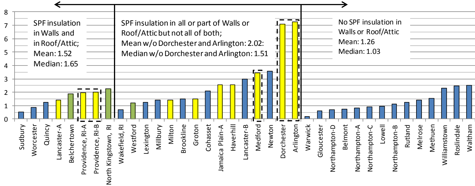
Figure 31. Post-DER ACH 50 results grouped use of SPF insulation in walls and roof
