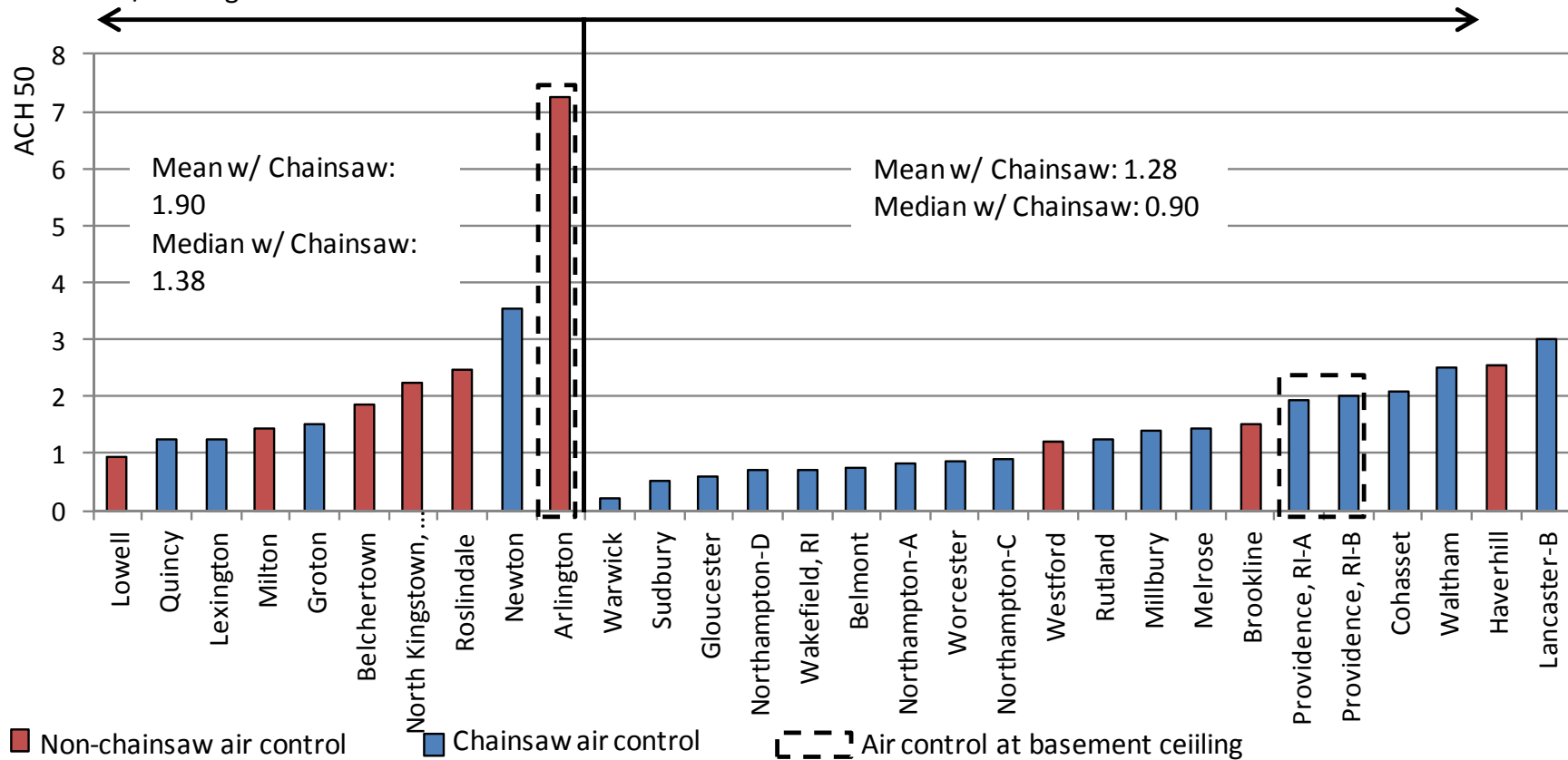
Figure 32. Post-DER ACH 50 results grouped by non-adhered/fully-adhered roof underlayment
