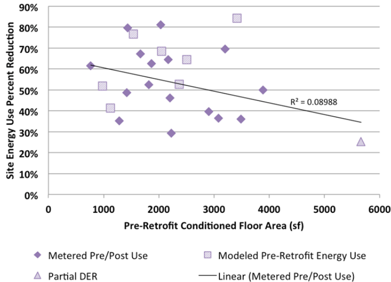
Figure 7. Site energy use percent reduction relative to pre-retrofit conditioned floor area
