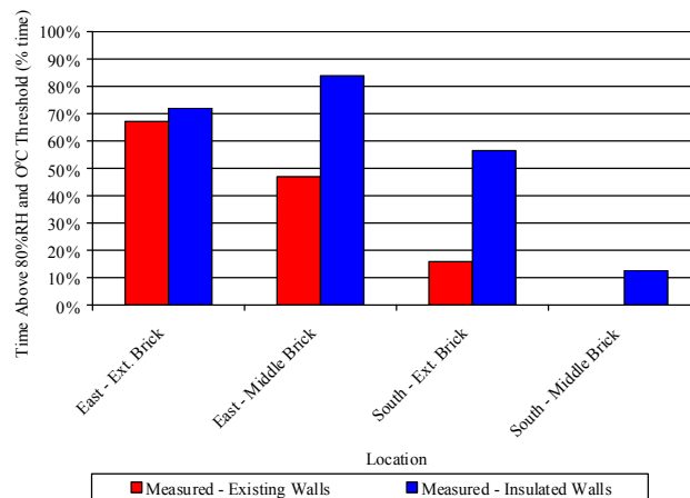
FIGURE 10: MEASURED TIME ABOVE CORROSION THRESHOLDS IN INSULATED AND EXISTING WALLS Insulated walls have significantly more time above corrosion thresholds than existing walls, increasing risks for embedded steel corrosion in insulated walls.
