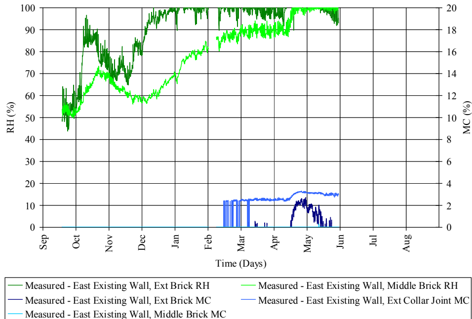
FIGURE 5: MEASURED RH AND MC IN EAST EXISTING WALL
