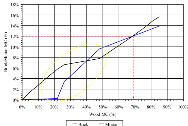
FIGURE 12: MOISTURE CONTENT CORRELATION – BRICK VS WOOD Corresponding Brick MC for given Wood MC reading. Wood sensors operate accurately in the range circled in yellow. Critical moisture content range for brick freeze-thaw analysis (and corresponding wood moisture content), shown with dotted red arrows.
