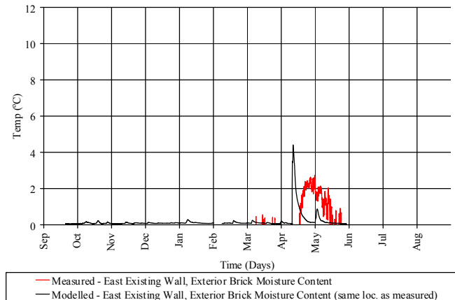
FIGURE 8: MEASURED AND MODELLED MOISTURE CONTENT IN EAST EXISTING WALL Moisture contents are generally similar, apart from severe spikes in modelled moisture content soon after rain events that are not observed in measured values. This discrepancy should be resolved with artificial wetting of the field sensors to test reaction time to wetting events.
