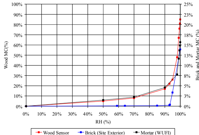
FIGURE 11: MOISTURE CONTENT CALIBRATION – WOOD AND BRICK Measurements taken during lab testing of wood sensor installed in brick, as done in the field.
