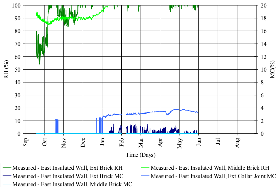
FIGURE 6: MEASURED RH AND MC IN EAST INSULATED WALL
