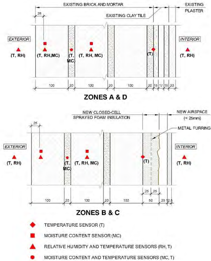
FIGURE 1: MOCK-UP WALL SECTIONS
