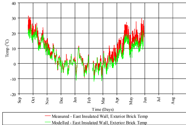
FIGURE 7: MEASURED AND MODELLED TEMPERATURES IN EAST INSULATED WALL Temperatures shown are similar between modelled and measured walls. Other locations also compare well.
