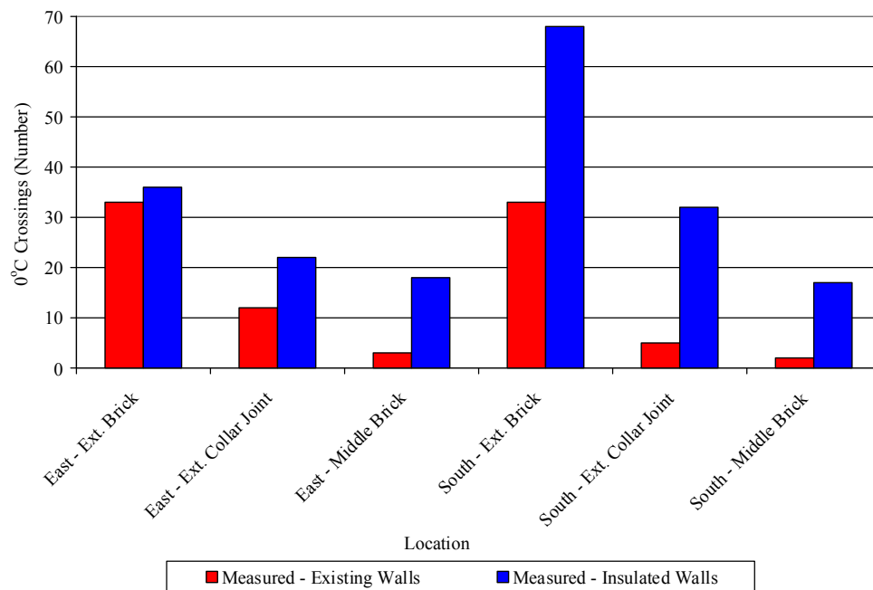
FIGURE 4: MEASURED ZERO-CROSSINGS IN INSULATED AND EXISTING WALLS This figure illustrates climate conditions relevant to freeze-thaw cycles. All insulated walls have an increase in the number of zero crossings, particularly the South elevation due to impacts from solar radiation. There were no hours when freeze thaw cycles were observed (when a zero crossing occurred and moisture contents were also above 85% of free water saturation).
