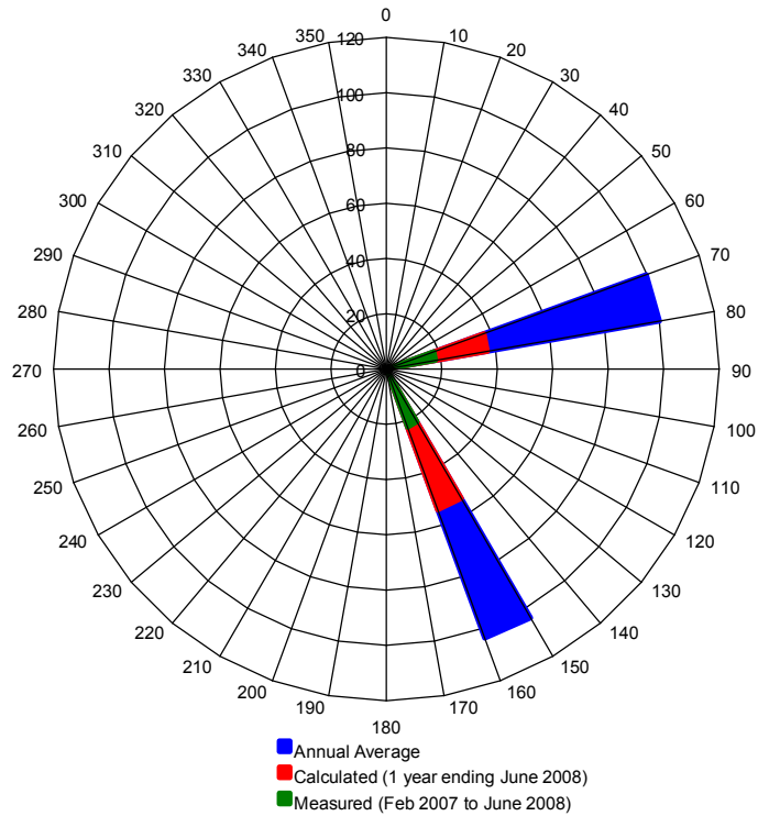
FIGURE 2: WIND-DRIVEN RAINFALL ON TEST WALLS
