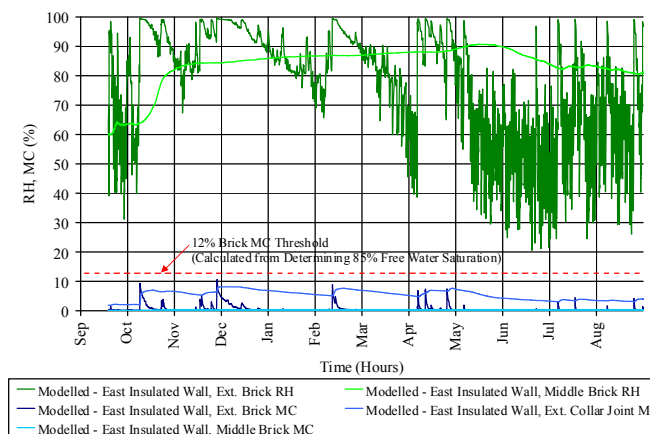
FIGURE 9: MODELLED RH AND MC IN EAST INSULATED WALL Brick moisture content in most severe modelled case is 10.6%, which is below the 12% MC freeze-thaw threshold.
