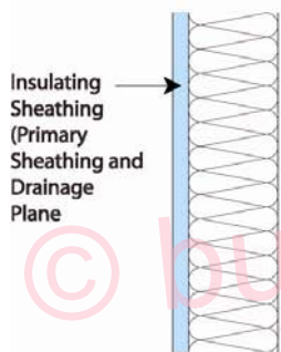
Wall Section 4
