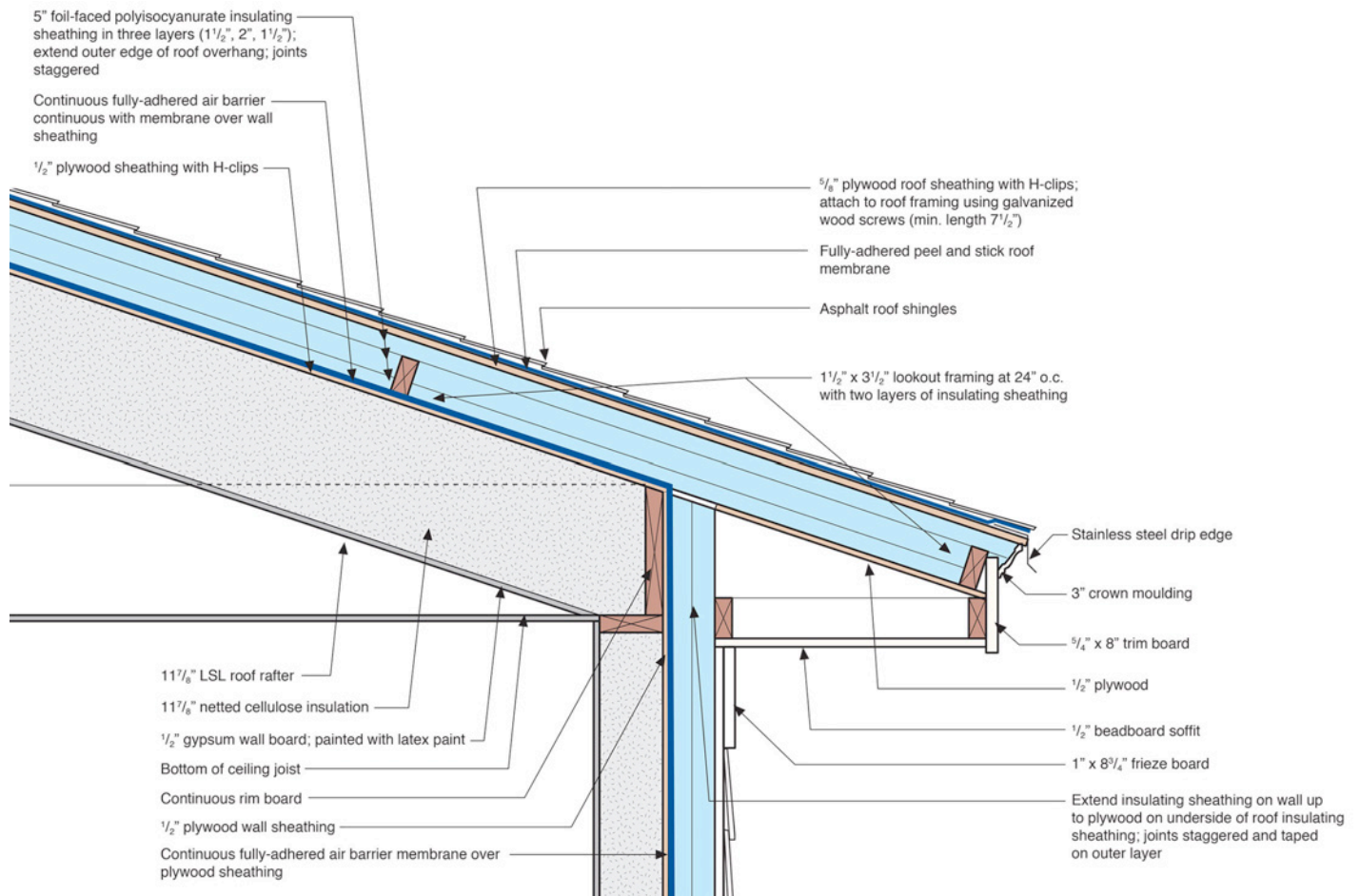
Figure 1 – Roof Assembly: Note the continuity of the water control layer, air control layer, vapor control layer and the thermal control layer. The “lookout” framing for the overhang is embedded in the rigid insulation. You want a higher R-value roof than this? Easy. Add another layer of rigid insulation. Or two layers. Don't like the cellulose in the cavities? Use fiberglass. Or use low density or high-density foam. Whatever.
