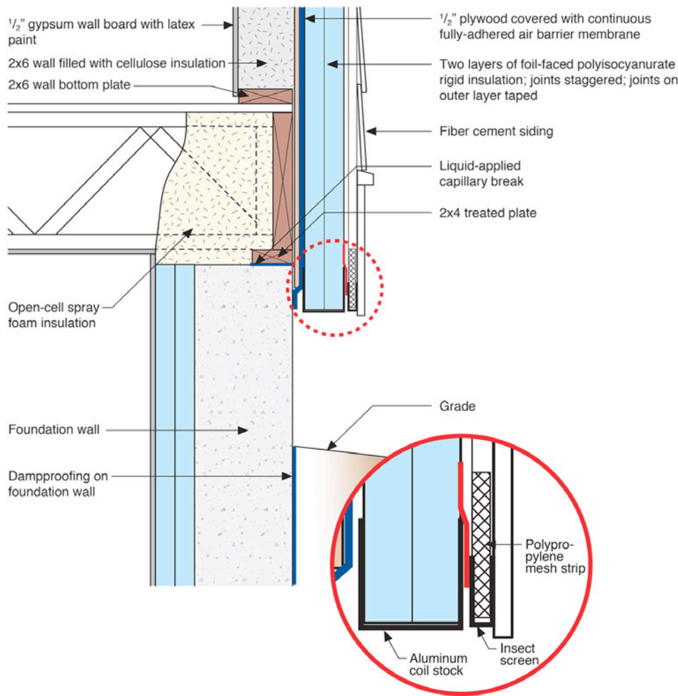
Figure 3 – Top of Foundation: Note that the fully-adhered membrane is sealed to the top of the exterior face of the concrete foundation wall. The membrane will have to be sealed with a mastic or a primer. Also note the physical protection of the bottom of the continuous insulation. This is absolutely necessary to deal with critters. Also note the insect screening.
