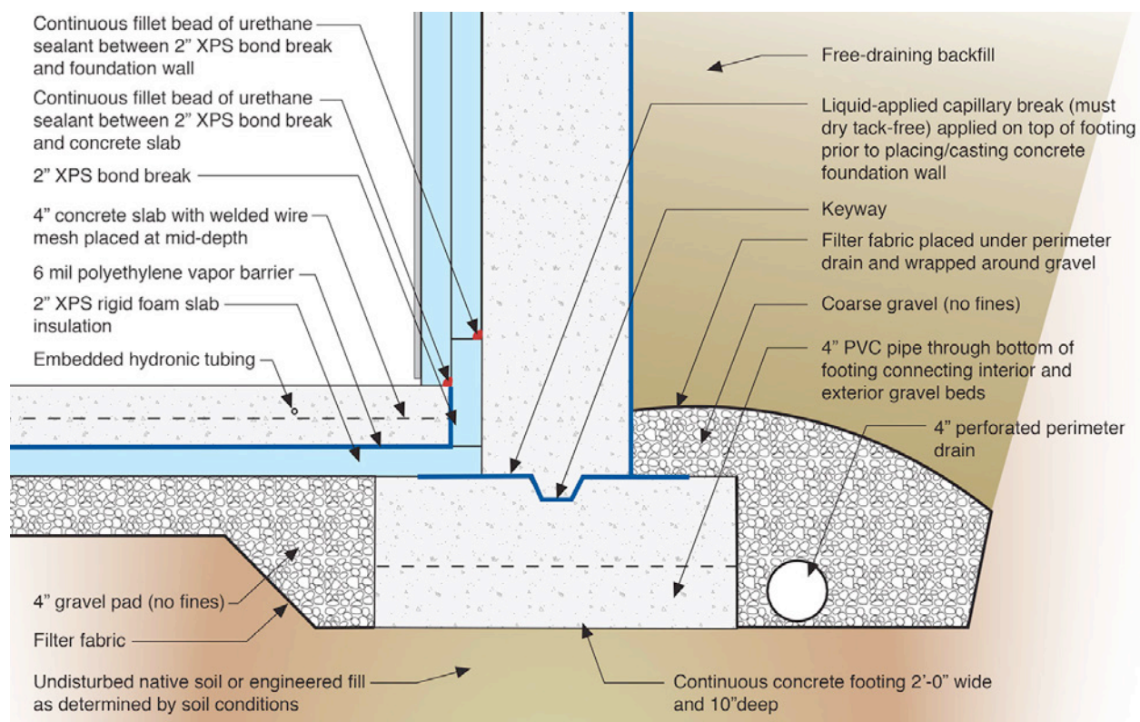
Figure 4 – Bottom of Foundation: Note the capillary break at the top of the footing. Also, note the two “red” sealant beads. They are absolutely necessary to create an airtight seal between the basement slab and the interior of the perimeter concrete foundation wall. Also note the filter fabric under the gravel pad. Not standard, but a really good idea.
