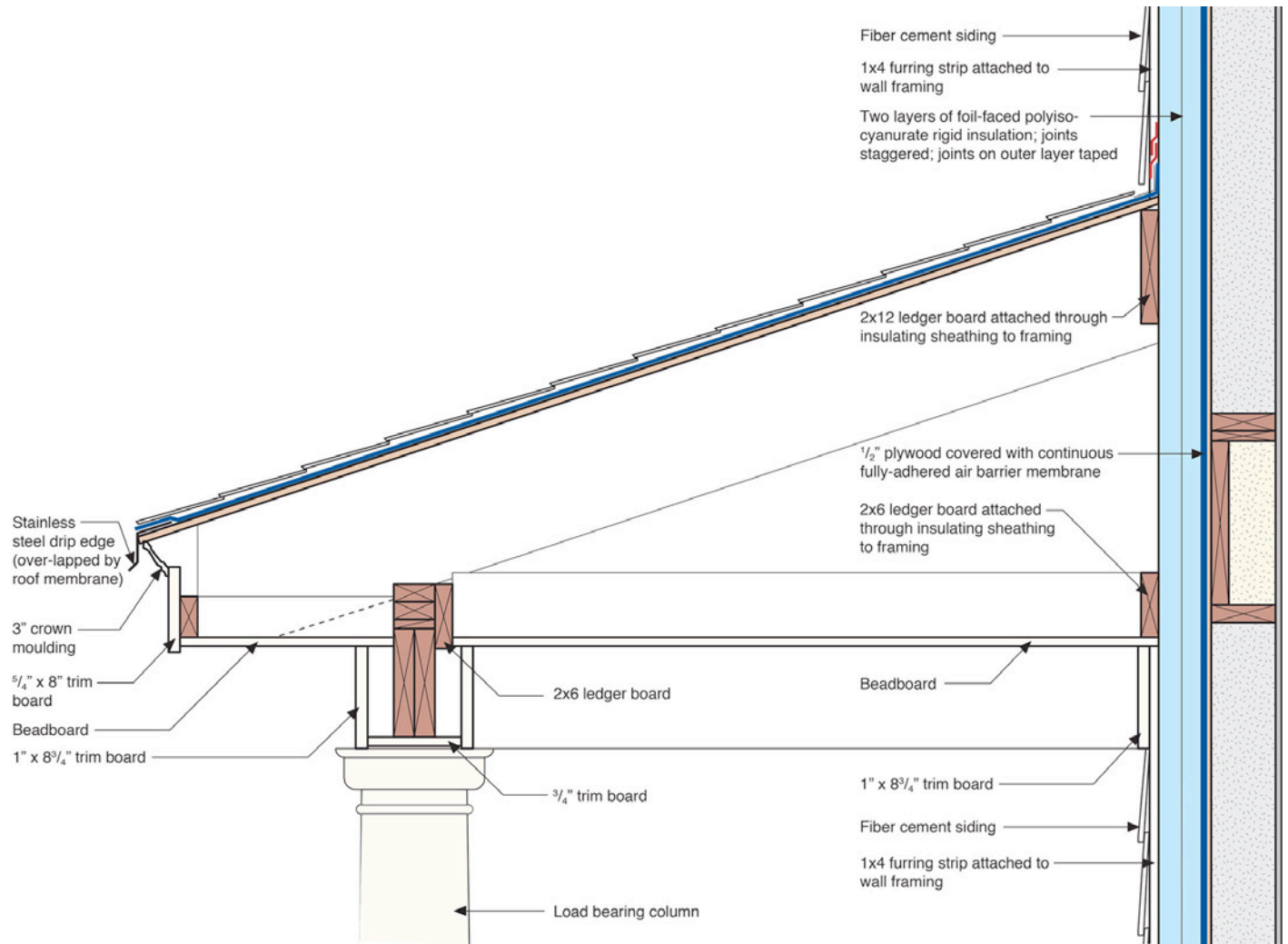
Figure 2 – Wall Assembly: Note that the “hood” framing does not penetrate the layers of exterior continuous insulation. Further note that the roof is flashed to the exterior face of the rigid insulation. If rockwool is used then the roof would need to be flashed to the exterior face of the fully-adhered membrane. You want a higher R-value? Add another layer of continuous insulation.
