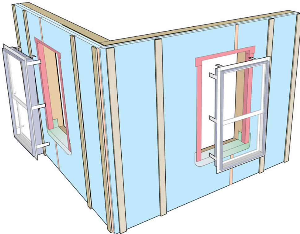
Figure 6 - Window Installation: Note the mounting brackets attached to standard flanged windows. Mounting brackets for masonry openings are used. Also note the pan flashing. The window is waterproofed to the face of the exterior sheathing. This detail remains the same for all of the various continuous insulation types. One caveat here: with rockwool, you will have to use unflanged windows and a 2 stage joint since the water control layer is the fully-adhered membrane not the exterior face of the continuous insulation as is the case with isocyanurate, XPS and EPS.
